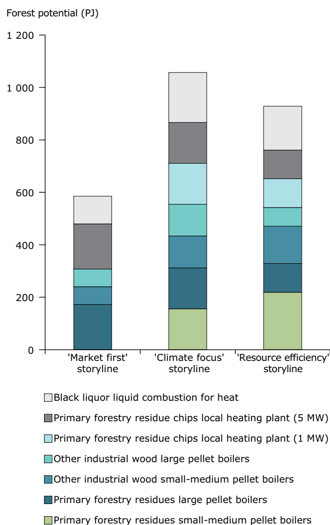
Figure 5.7 Forest potential (PJ) and technology mix per storyline in 2020
