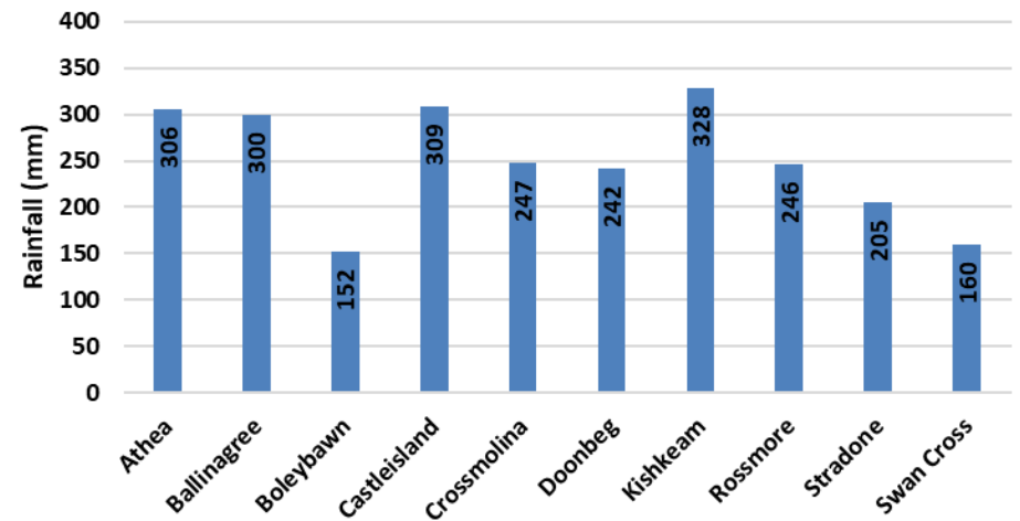
Cumulative Rainfall 2024
