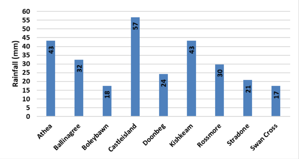
Cumulative Rainfall 01 to 14 of Jan.
