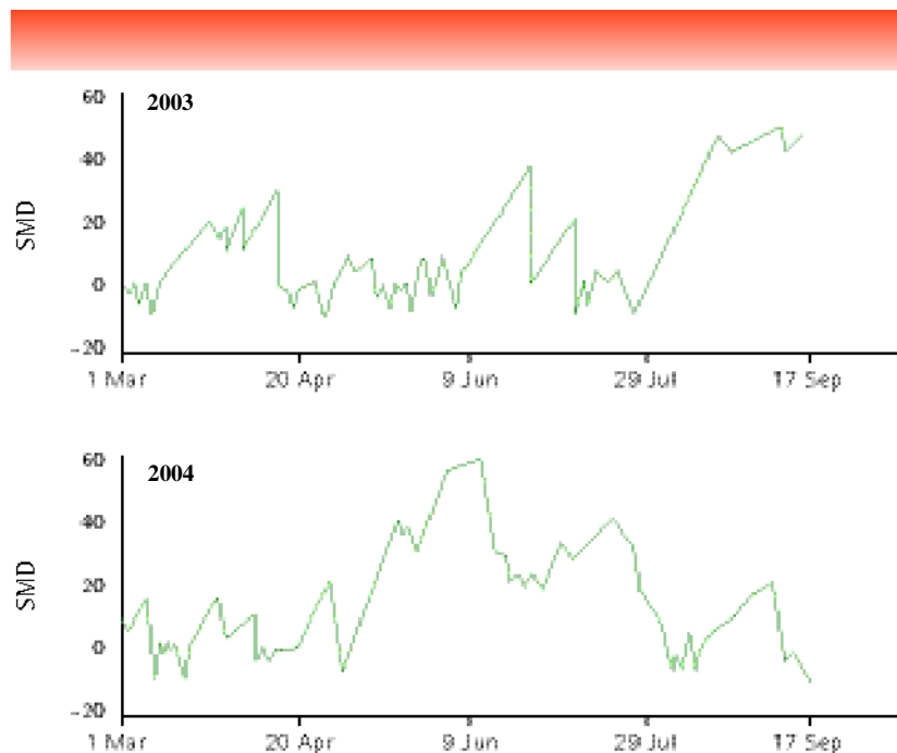
Figure 7. Soil moisture deficits at Solohead between March and September 2003 and 2004: 0 = wet, 10 to 25 = good grass and grazing conditions, >25 = ground getting dry and hard, >50 = grass growth increasingly restricted, > 75 = drought conditions.
