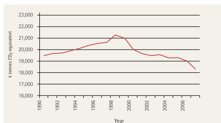
FIGURE 2: Trend in tonnes \text{CO}_2 equivalent from agriculture (1990 - 2007) (source: EPA, 2008).
