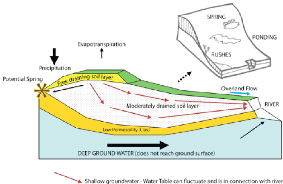
Figure 2. Illustration of how ground water interacts with surface water and the ground surface. It includes a simple sketch showing typical features on moderately to poorly drained land e.g. spring, seepage, ponding and rushes in a shallow water table area
