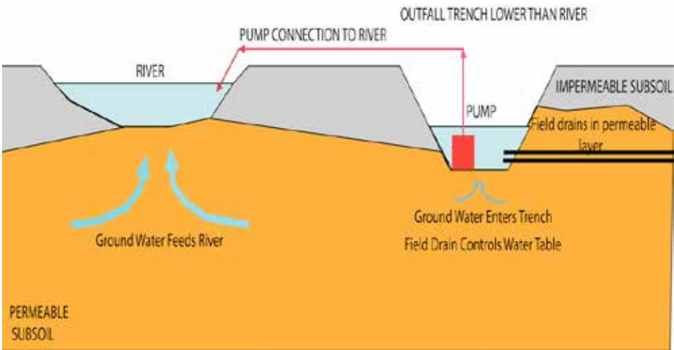
Figure 5. An example of a pumped outfall
