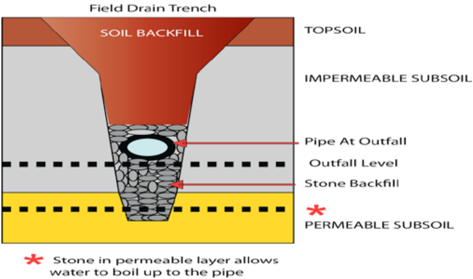
Figure 4. Targeting the permeable layer
