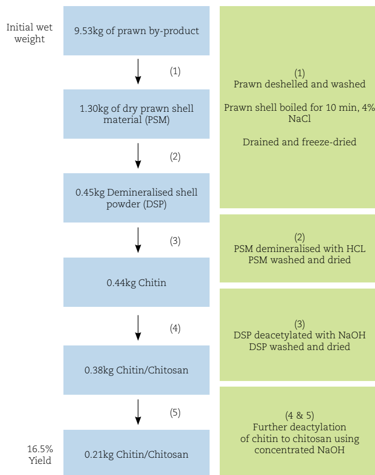
Figure 2. Generation of chitosan from prawn shell waste material.
