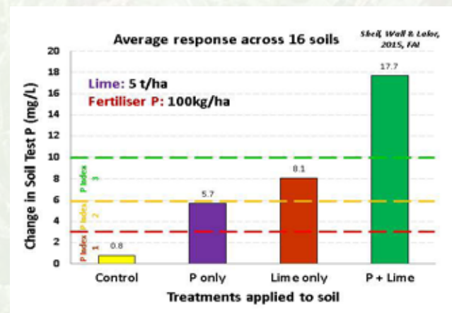
Figure 2. Average change in soil test P (Morgan's) across 16 soils (av. pH 5.2) treated with Lime (5 t/ha of lime), P fertiliser (100 kg/ha of P), and P + Lime and incubated over 12 months in controlled conditions
