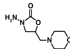
3-Amino-5-morpholinomethyl-2-oxazolidinone
