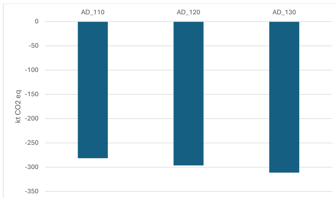
Figure 17: Decline in N2O Emission (in CO2 Eq.) by 2030 under the three scenarios
